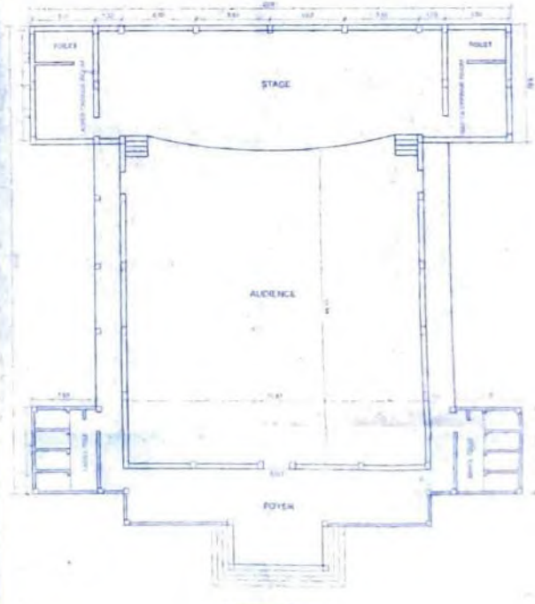
PLAN OF AUDITORIUM
